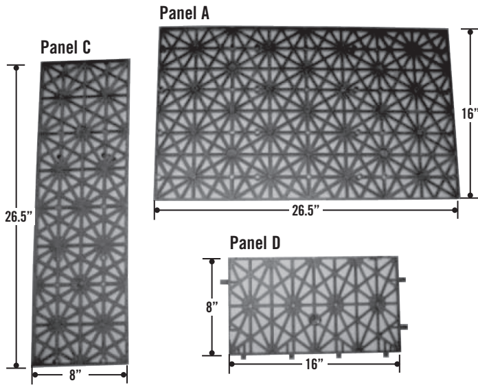
Small Matrix consists of 8 panels: 2 "A", 2 "C" and 4 "D" (see chart below for dimensions)
