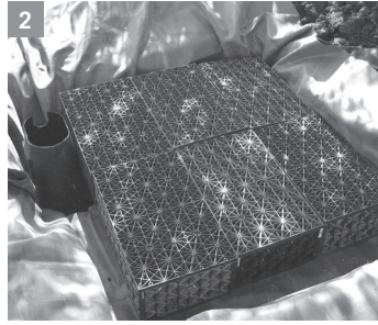
Step 2 – install the Snorkel™ Vault, Centipede™ Module and the AquaBlox™ Water Matrix System.
