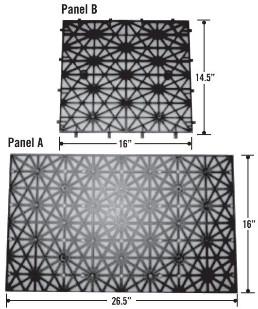
Large Matrix consists of 8 panels: 4 "A" and 4 "B" (see chart below for dimensions)
